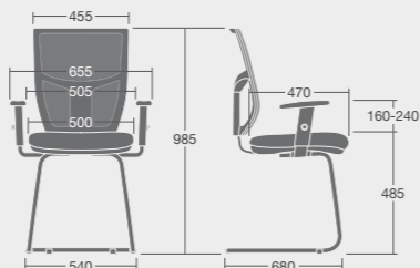
TPMC/1D: Overall Dimensions: 655w x 680d x 985h
