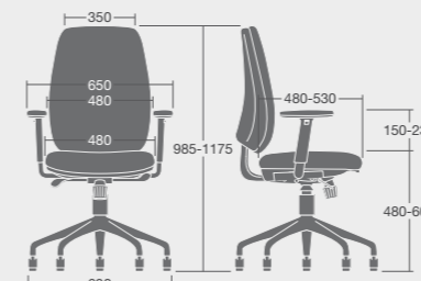
LOR/U/3D: Overall Dimensions: 690w x 690d x 1175h
