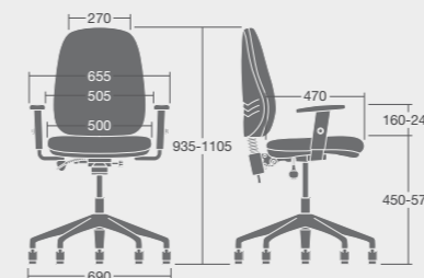
TEP/1D: Overall Dimensions: 690w x 690d x 1105h
