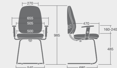
TEPC/1D: Overall Dimensions: 655w x 680d x 985h
