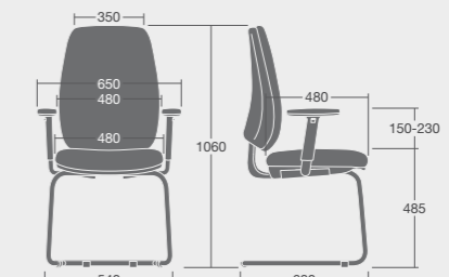
LORC/U/3D: Overall Dimensions: 650w x 680d x 1060h
