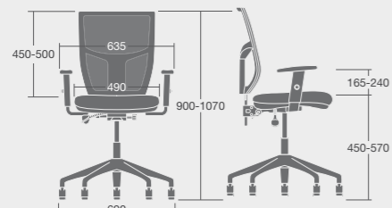
TPM/1D: Overall Dimensions: 690w x 690d x 1070h
