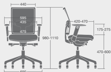
LOR/BM/1D: Overall Dimensions: 690w x 690d x 1110h
