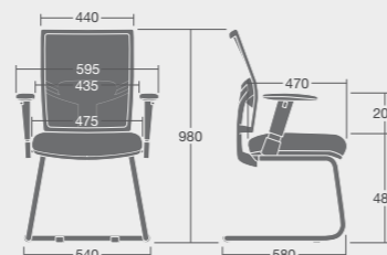
LORC/BM/FA: Overall Dimensions: 595w x 580d x 980h
