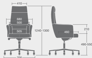
VENHB: Overall Dimensions: 700w x 700d x 1300h
