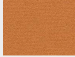
Measure CSE27
