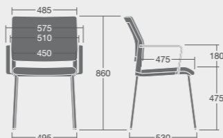
ISITL/LA: Overall Dimensions: 575w x 580d x 860h
