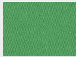
Event CSE18
