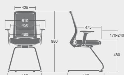
VIDC/1D: Overall Dimensions: 610w x 560d x 980h
