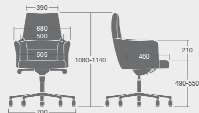
VEN: Overall Dimensions: 700w x 700d x 1140h
