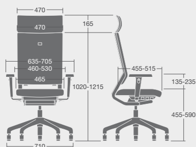
ISIT/UH/4D2: Overall Dimensions: 710w x 710d x 1380h
