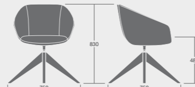
LUMSWWL: Overall Dimensions: 750w x 750d x 830h
