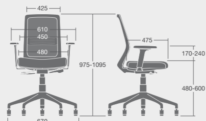
VID/1D: Overall Dimensions: 670w x 670d x 1095h
