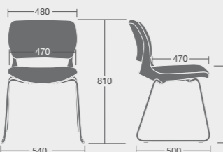
ACESB : Overall Dimensions: 540w x 500d x 810h
